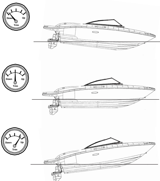
EFFECTS OF POWER TRIM (FIG. 2.8.1)
