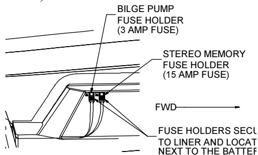
STEREO MEMORY/BILGE PUMP FUSES (FIG. 6.4.1)
