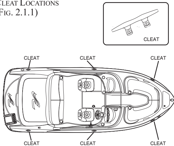
BOW AND STERN EYE LOCATIONS (FIG. 2.1.2)
