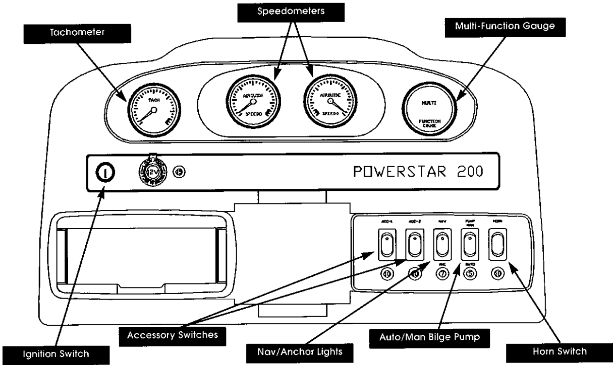
Mercury Instrument Panel (Standard)
