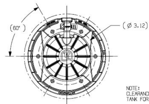
DETAIL B SCALE 1:2 VALVE ORIENTATION SHOWN AS REFERENCE
