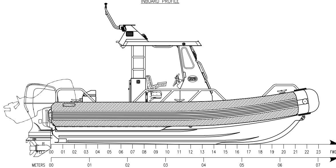
OUTBOARD PROFILE
