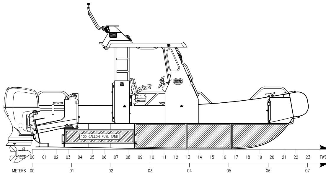
INBOARD PROFILE
