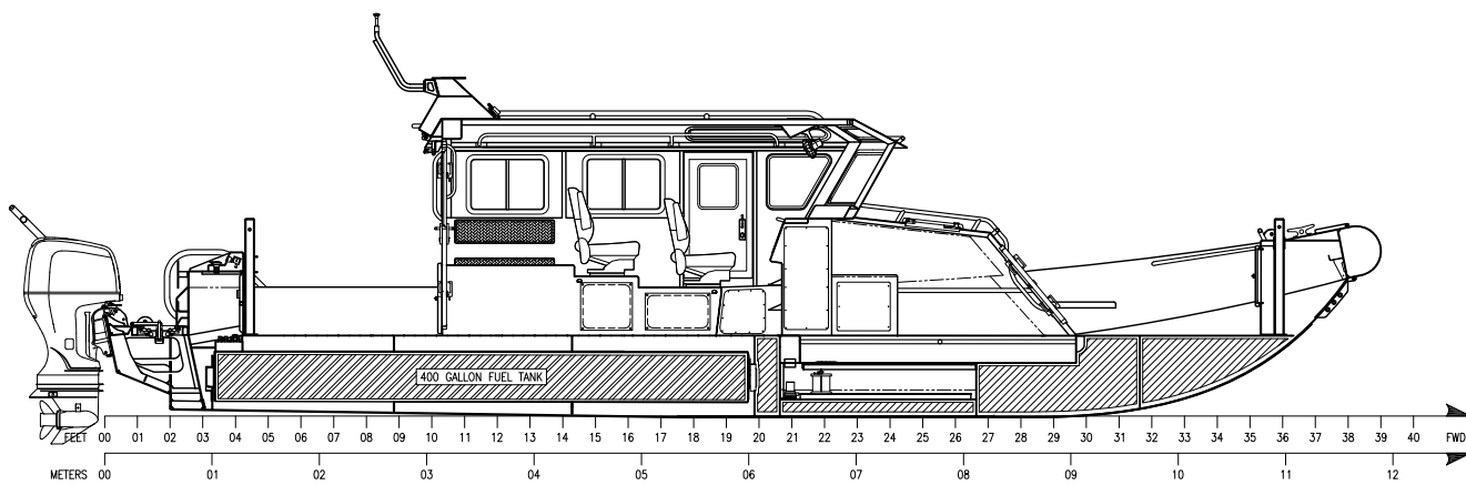
INBOARD PROFILE
