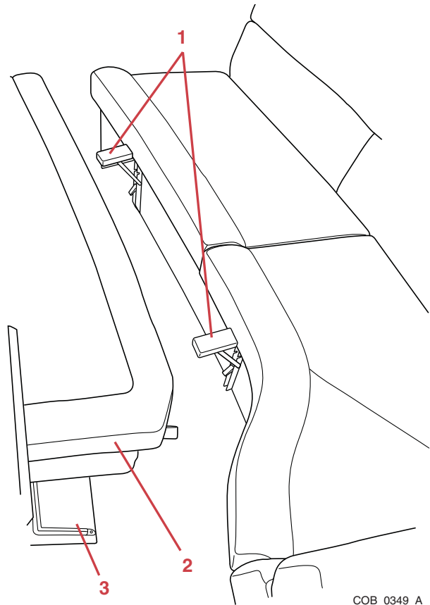
1 – Cabin Filler Supports 2 – Cabin Filler Slides from Stowed and Deployed Positions 3 – Cabin Filler Door
