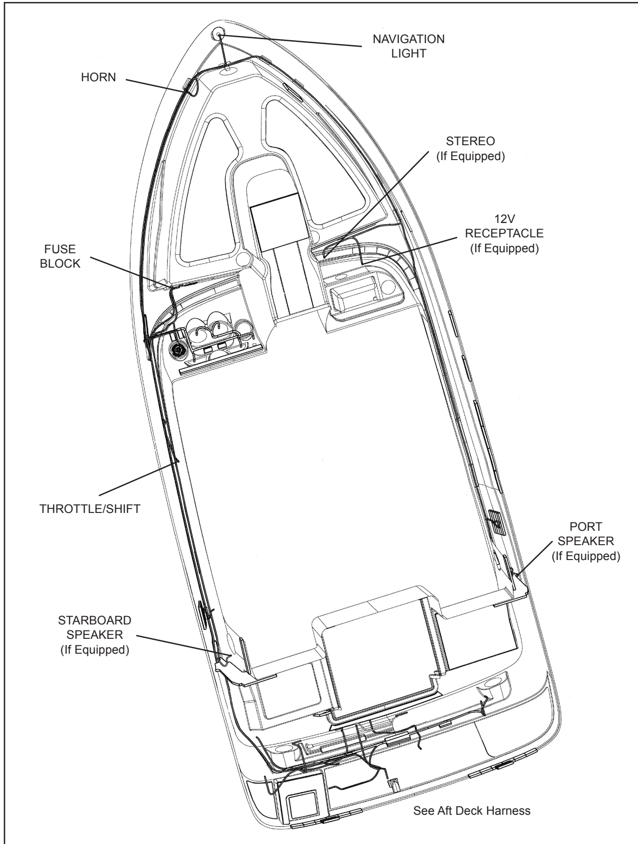
DECK UNDERSIDE
