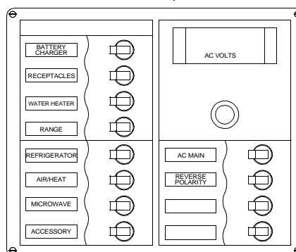
110-VOLT AC MASTER PANEL (SINGLE SHORE POWER)
