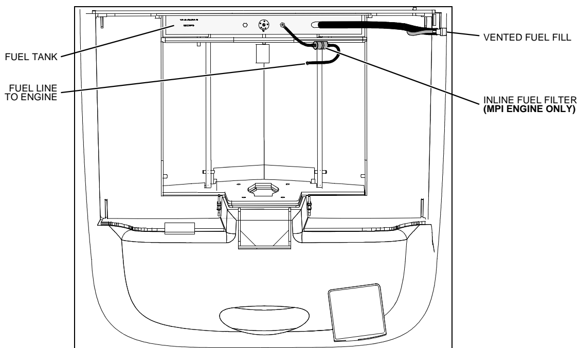
GAS ENGINE FUEL LINE ROUTING (IF EQUIPPED)
