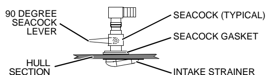
SEAWATER INTAKE VALVE (SEACOCK) COMPONENTS (TYPICAL)
